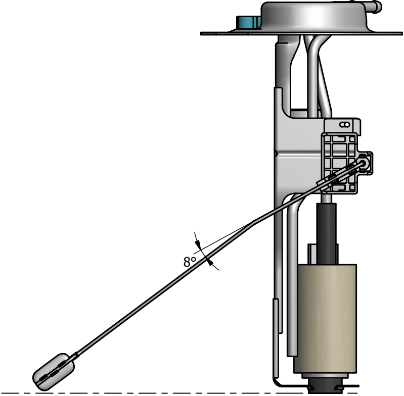
WITH MODIFIED FLOAT ARM
