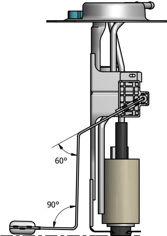
WITH EXISTING FLOAT ARM
